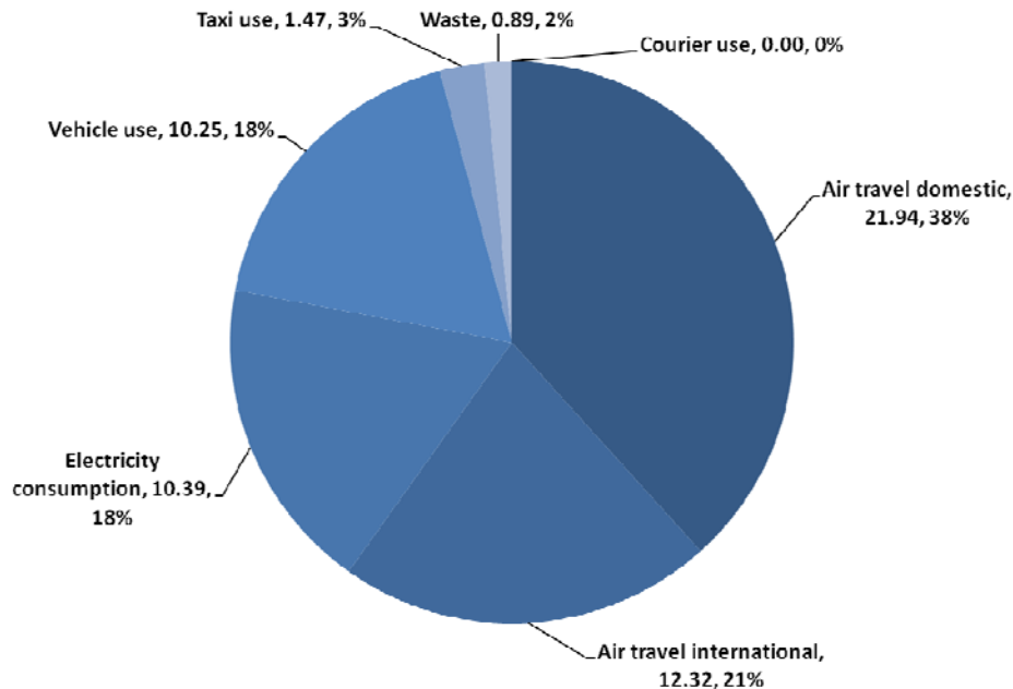
Figure 1: GHG emissions sources.
